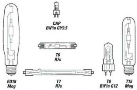
Metal Halide Lamps
